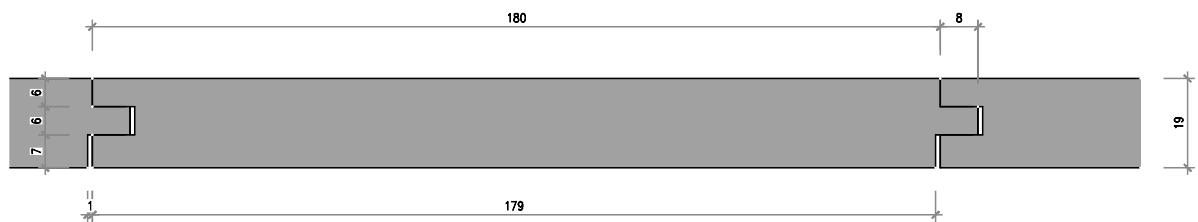
Nr. 4145-M N+K 19/180 mm, Kamm 8 mm lang parallel
